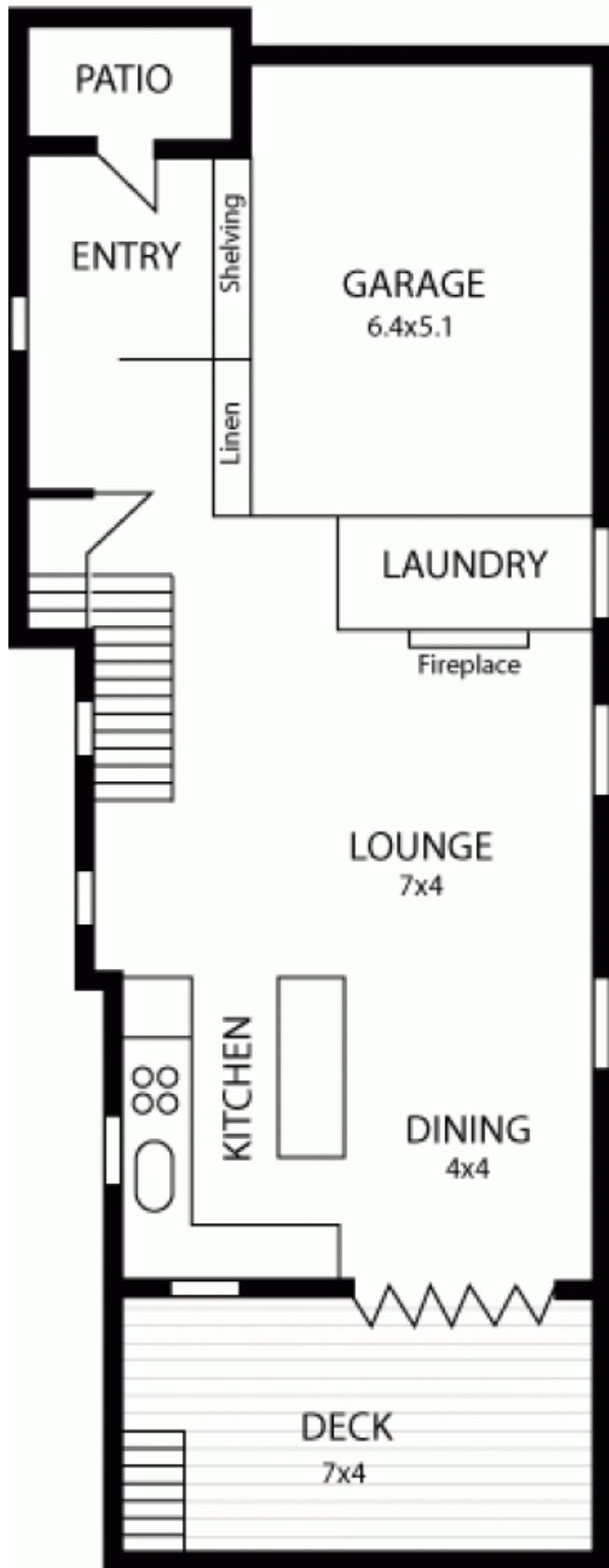
GROUND FLOOR
